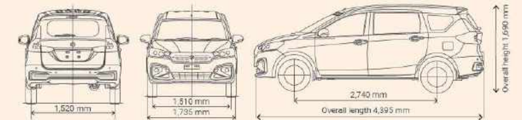
The drawings shown are general specifications of the vehicle.
